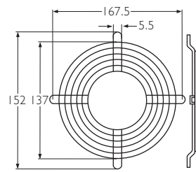
LZ27 Welded steel guard, bright zinc. 7xxx series fans
